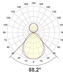
PPS1200125_PD-26W-4000K
