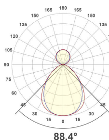
PPS1200125_PD-30W-4000K
