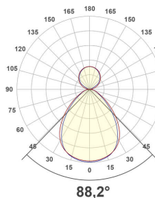
PPS1200125_PD-26W-3000K
