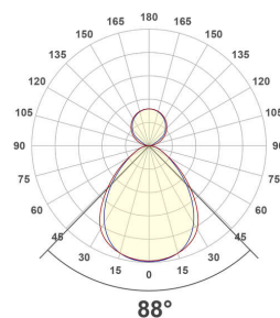
PPS1200125_PD-30W-mix
