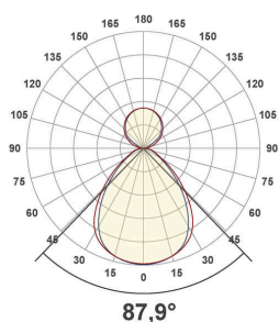
PPD1500125_PD-37W-4000K
