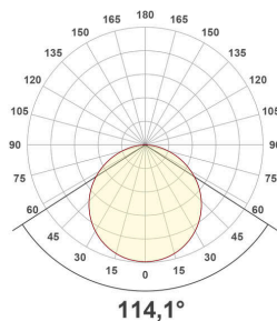
LTWR220125_PD-5700K
