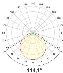
LTWR220125_PD-2700K
