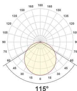
LDQ170125_PD-3000K
