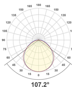
FLS120125_PD-35W-4000K
