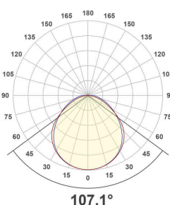
FLS120125_PD-30W-3000K
