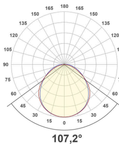
FLD150125_PD-45W-4000K
