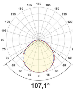
FLD150125_PD-45W-3000K
