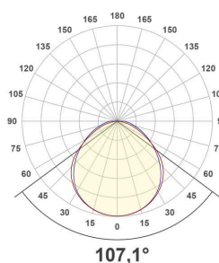
FLD120125_PD-35W-3000K
