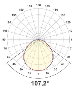
FLD120125_PD-35W-4000K
