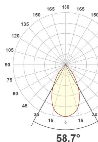
ET54504925_PD-4000K
