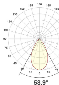
ET54504925_PD-5700K
