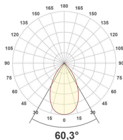
ES54504125_PD-26W-3000K
