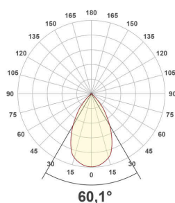
ES54504125_PD-34W-4000K
