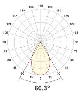
ES54504125_PD-34W-3000K
