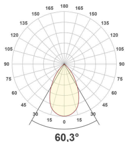
ES54504125_PD-20W-4000K
