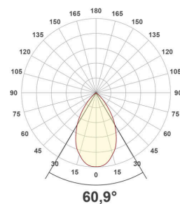
ES54280125_PD-28W-5700K
