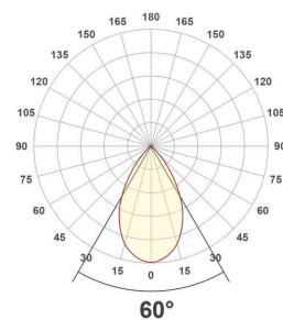
ES54280125_PD-24W-4000K
