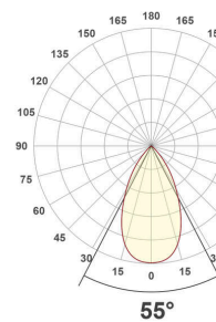
ES54204925_PD-20W-5700K
