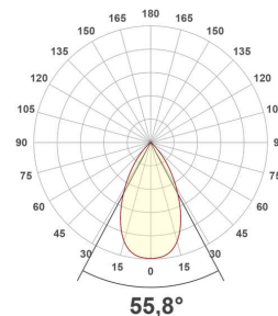
ES54200925_PD-16W-4000K
