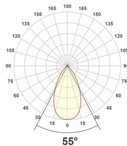
ES54200925_PD-16W-3000K
