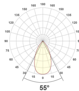
ES54200925_PD-18W-5700K
