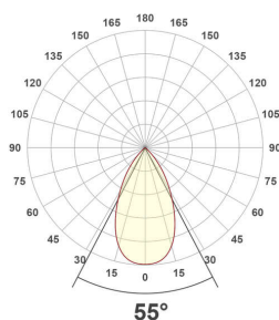
ES54200925_PD-18W-3000K
