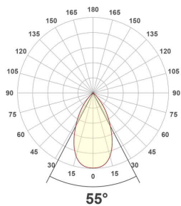
ES54200925_PD-20W-3000K
