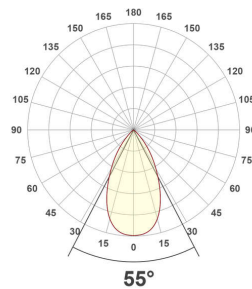
ES54200925_PD-20W-5700K
