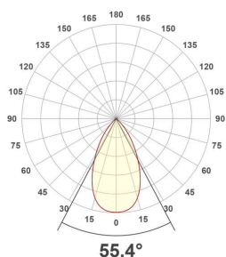
ES54200925_PD-16W-5700K
