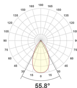
ES54200925_PD-18W-4000K
