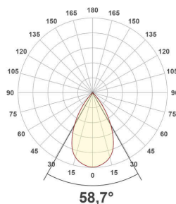
ES54104125_PD-8W-3000K
