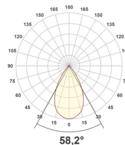
ES54104125_PD-8W-4000K
