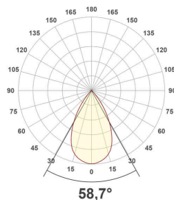
ES54104125_PD-8W-5700K
