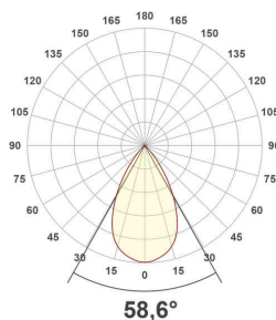
ES54104125_PD-6W-5700K
