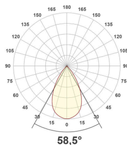
ES54104125_PD-6W-4000K
