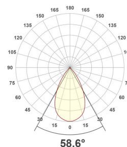
ES54100925_PD-8W-4000K
