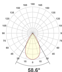
ES54100925_PD-6W-5700K
