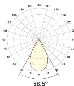
ES54100925_PD-6W-4000K
