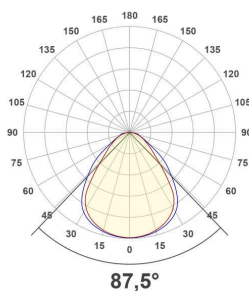
EPSU150125_PD-37W-3000K
