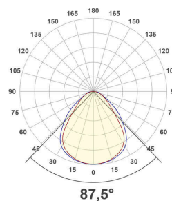
EPSU150125_PD-42W-4000K
