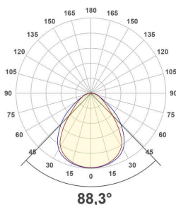
EPSU150125_PD-42W-3000K
