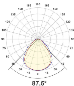
EPSU150125_PD-37W-4000K
