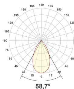
ED54504925_PD-4000K
