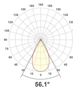
ED54104125_PD-4000K
