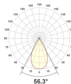
ED54104125_PD-3000K
