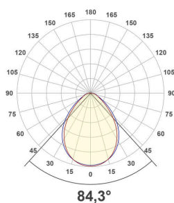
APTU150125_PD-54W-4000K
