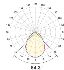
APTU150125_PD-54W-3000K
