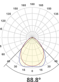
APSU620125_PD-25W-mix
