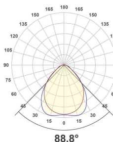
APSU620125_PD-33W-4000K
