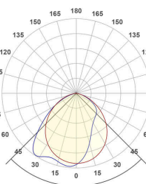
APS1200125AS_PD-17W-4000K
