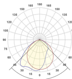
APS1200125AS_PD-30W-4000K
