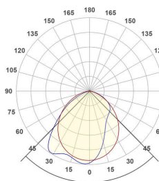
APS1200125AS_PD-26W-3000K
