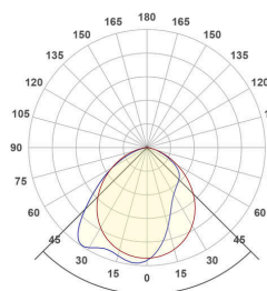
APS1200125AS_PD-22W-4000K
