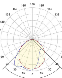
APS1200125AS_PD-26W-4000K
