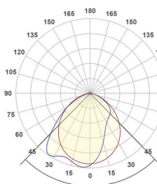
APS1200125AS_PD-22W-3000K
