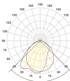
APS1200125AS_PD-30W-3000K
