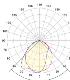
APS1200125AS_PD-17W-3000K
